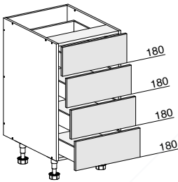
4 EQUAL DRAWER
