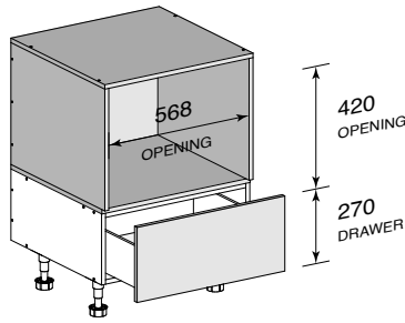
UB MICROWAVE CABINET (Space Only) with 270 Drawer
