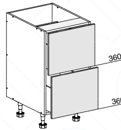
2 EQUAL DRAWER
