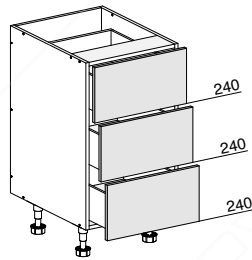
3 EQUAL DRAWER
