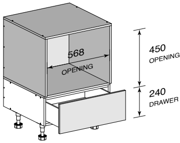
UB MICROWAVE CABINET (Space Only) with 240 Drawer
