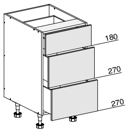
3 DRAWER (1 CUTLERY DRAWER, 2 POT DRAWERS)
