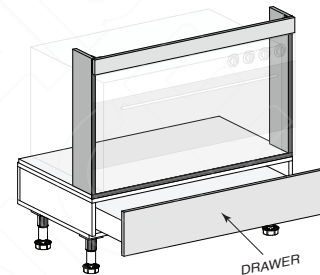
UB OVEN 900 Wide with Drawer
