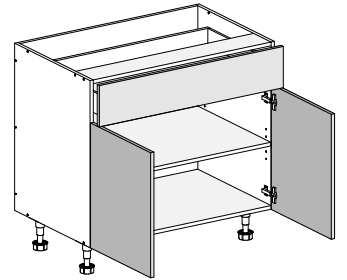
1 DRAWER, 2 DOOR
